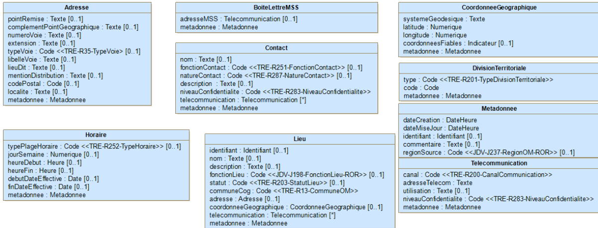
Figure 10 Classes communes
