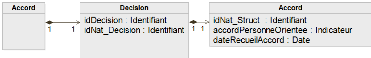
Figure 12 Flux 2 - Accord
