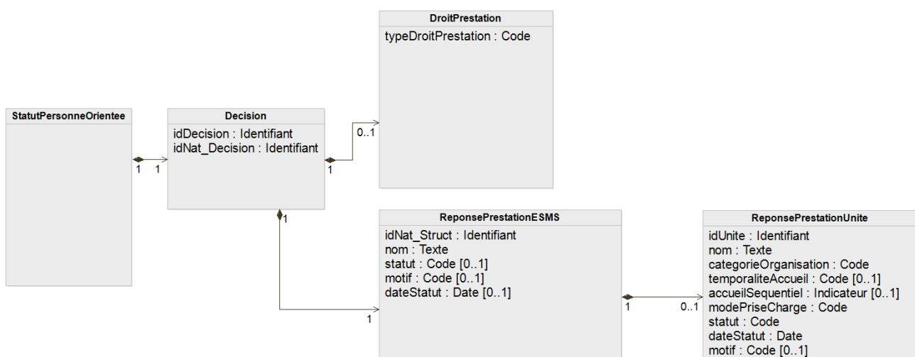
Figure 14 Flux 4 – StatutPersonneOrientee
